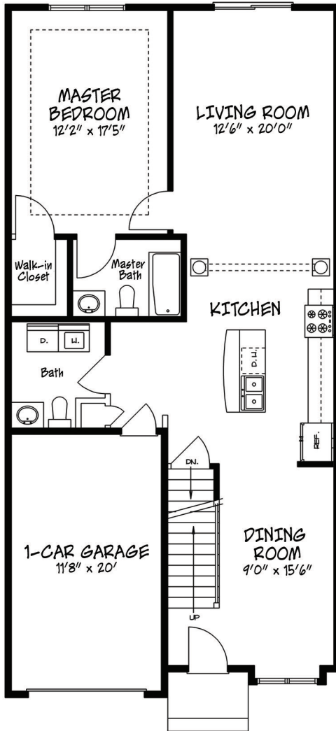
FIRST FLOOR PLAN Living Area: 1,123 SF | Garage Area: 259 SF
